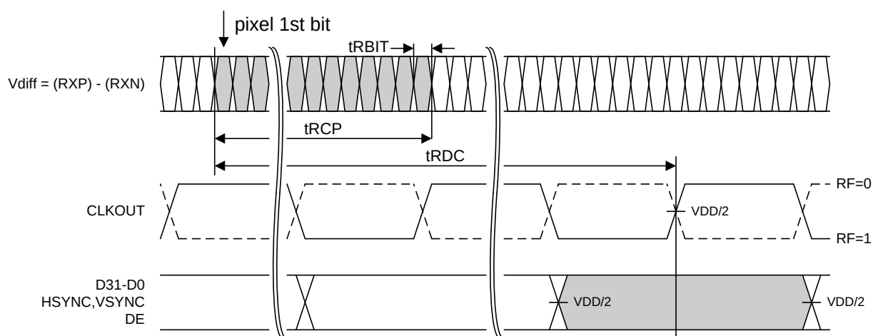
Figure 26. THCV236-Q Latency
