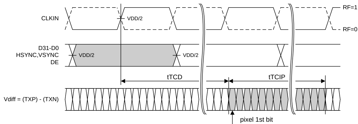
Figure 25. THCV235-Q Latency
