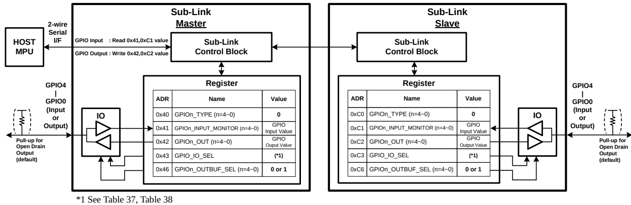
Figure 15. Programmable GPIO
