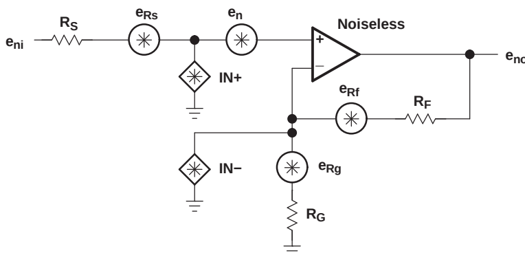
Figure 52. Noise Model
