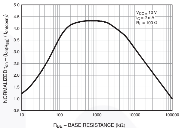
Figure 10. Normalized t_{\text{on}} vs. R_{BE}
