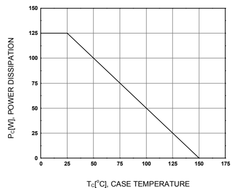
Figure 6. Power Derating
