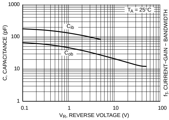
Figure 12. Capacitance
