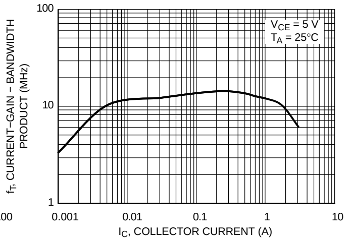
Figure 13. Current-Gain-Bandwidth Product
