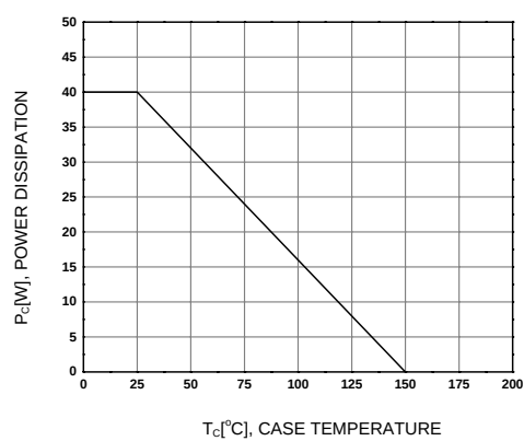
Figure 4. Power Derating
