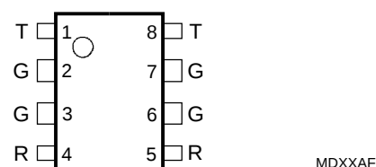
P PACKAGE (TOP VIEW)
