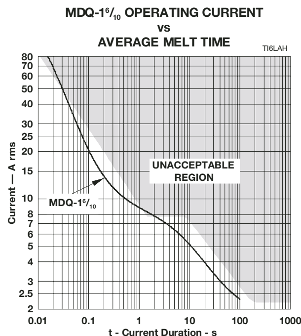
Figure 17. MDQ-1 6 / 10 Current-Time
