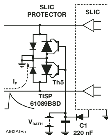
Figure 8. Positive Overvoltage Condition
