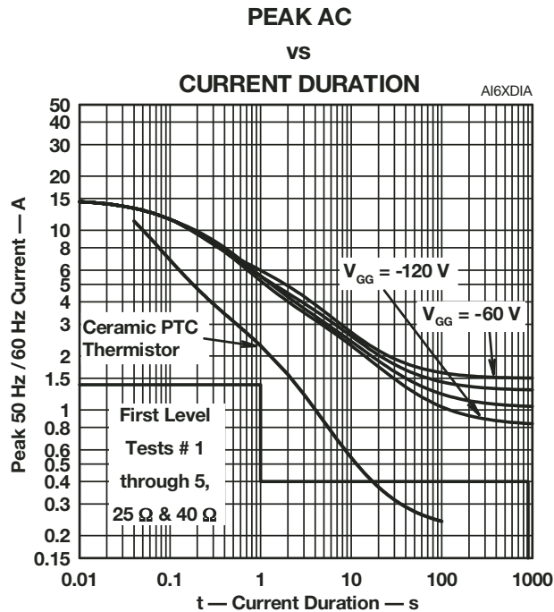
Figure 21. Ceramic PTC Thermistor
