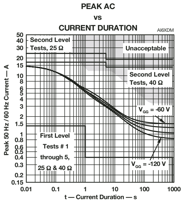
Figure 19. TISP61089BSD Overlay
