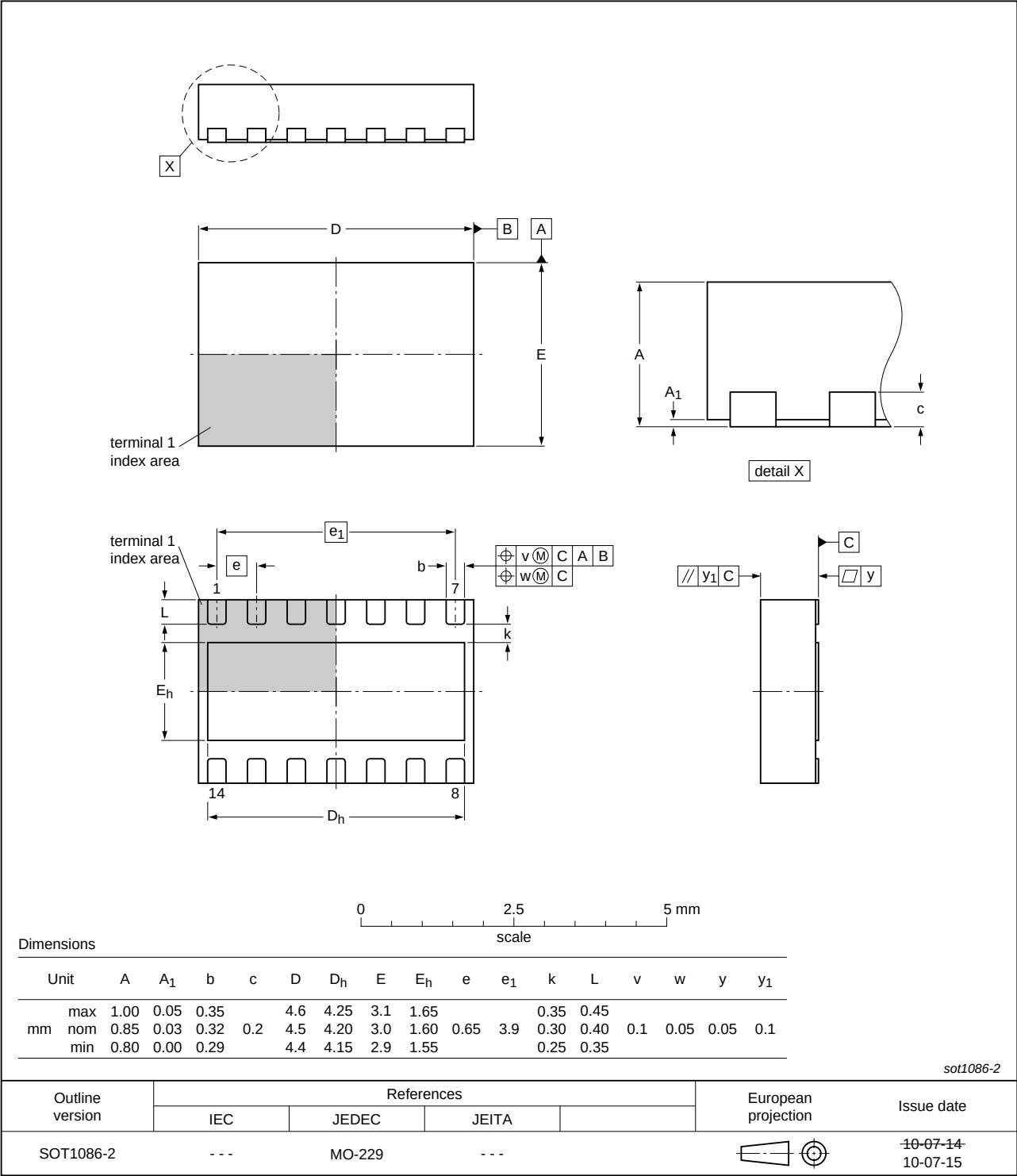
Fig 8. Package outline SOT1086-2 (HVSON14)
