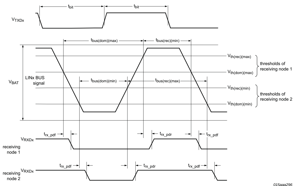
Fig 5. Timing diagram of LIN transceiver duty cycle
