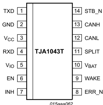
Fig 2. Pin configuration diagram: SO14
