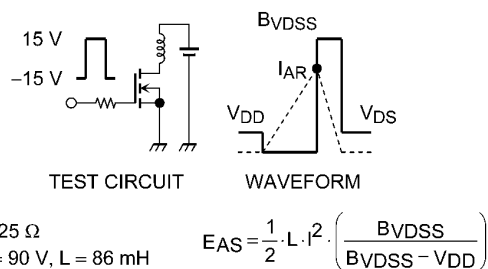
Fig. 8.16 Test Circuit/Waveform
