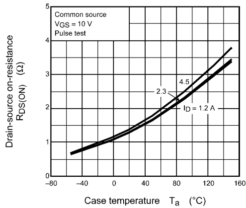
Fig. 8.7 R_{DS(ON)} - T_a
