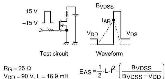
Fig. 8.16 Test Circuit/Waveform
