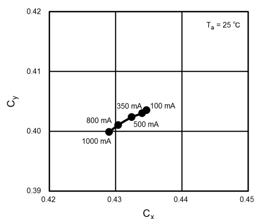
Fig. 8.4 Chromaticity - I_F
