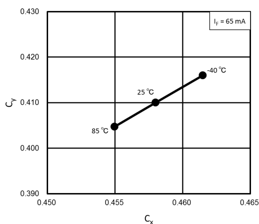
Fig. 8.5 Chromaticity - T_a
