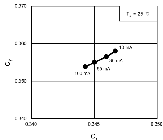
Fig. 8.4 Chromaticity - I_F
