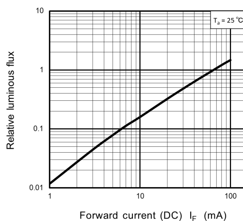
Fig. 8.2 Relative Luminous Flux - I_F
