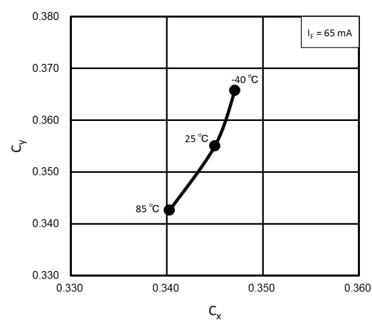
Fig. 8.5 Chromaticity - T_a
