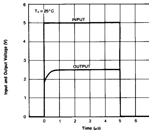
Figure 6. Pulse Response
