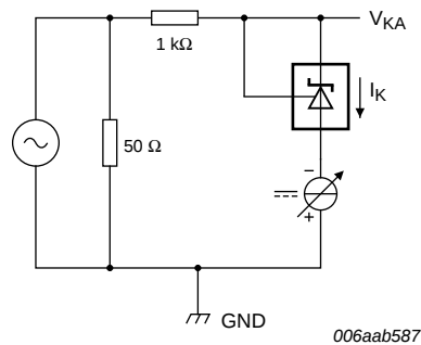
Fig 22. Test circuit to Figure 19 , Figure 20 and Figure 21
