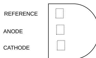
TO-92 TOP VIEW
