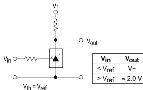
Fig 15 . Single-supply comparator with temperature-compensated threshold
