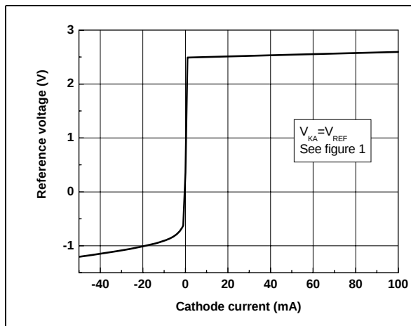
Figure 10. Reference voltage vs. cathode current
