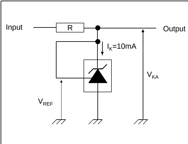
Figure 4. Test circuit for V_{KA} = V_{REF}
