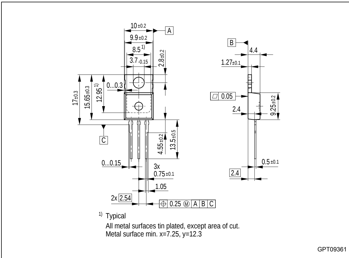
Figure 5 PG-TO220-3-1 (Plastic Transistor Single Outline)
