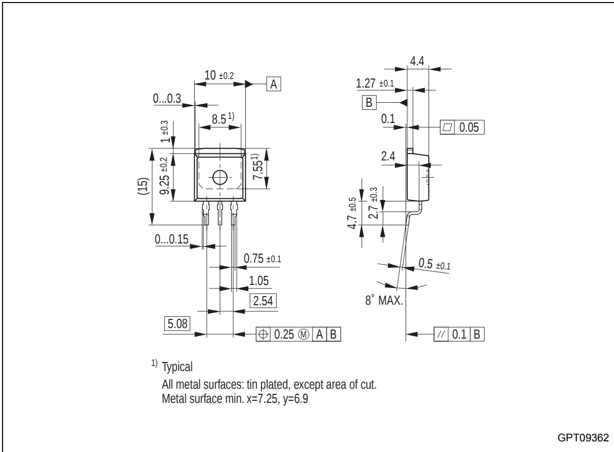
Figure 7 PG-T0263-3-1 (Plastic Transistor Single Outline)
