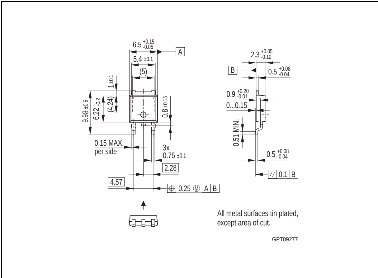
Figure 6 PG-T0252-3-11 (Plastic Transistor Single Outline)
