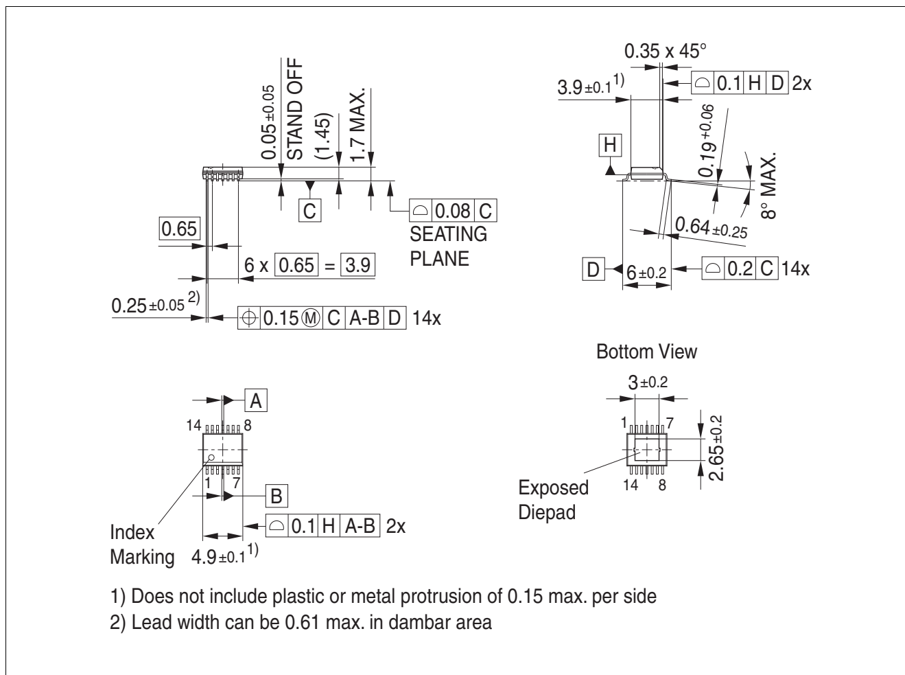
Figure 14 PG-SSOP-14 exposed pad
