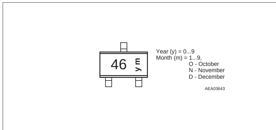
Figure 4 Marking TLE4946H
