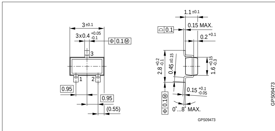
Figure 8 SC59
