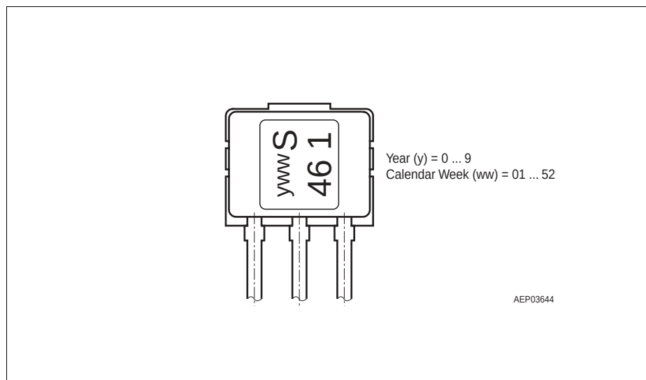
Figure 5 Marking TLE4946-1L
