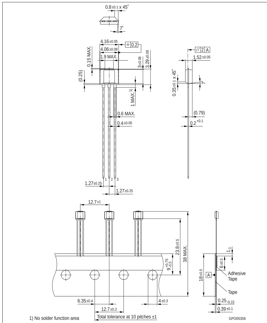
Figure 10 PG-SSO-3-2
