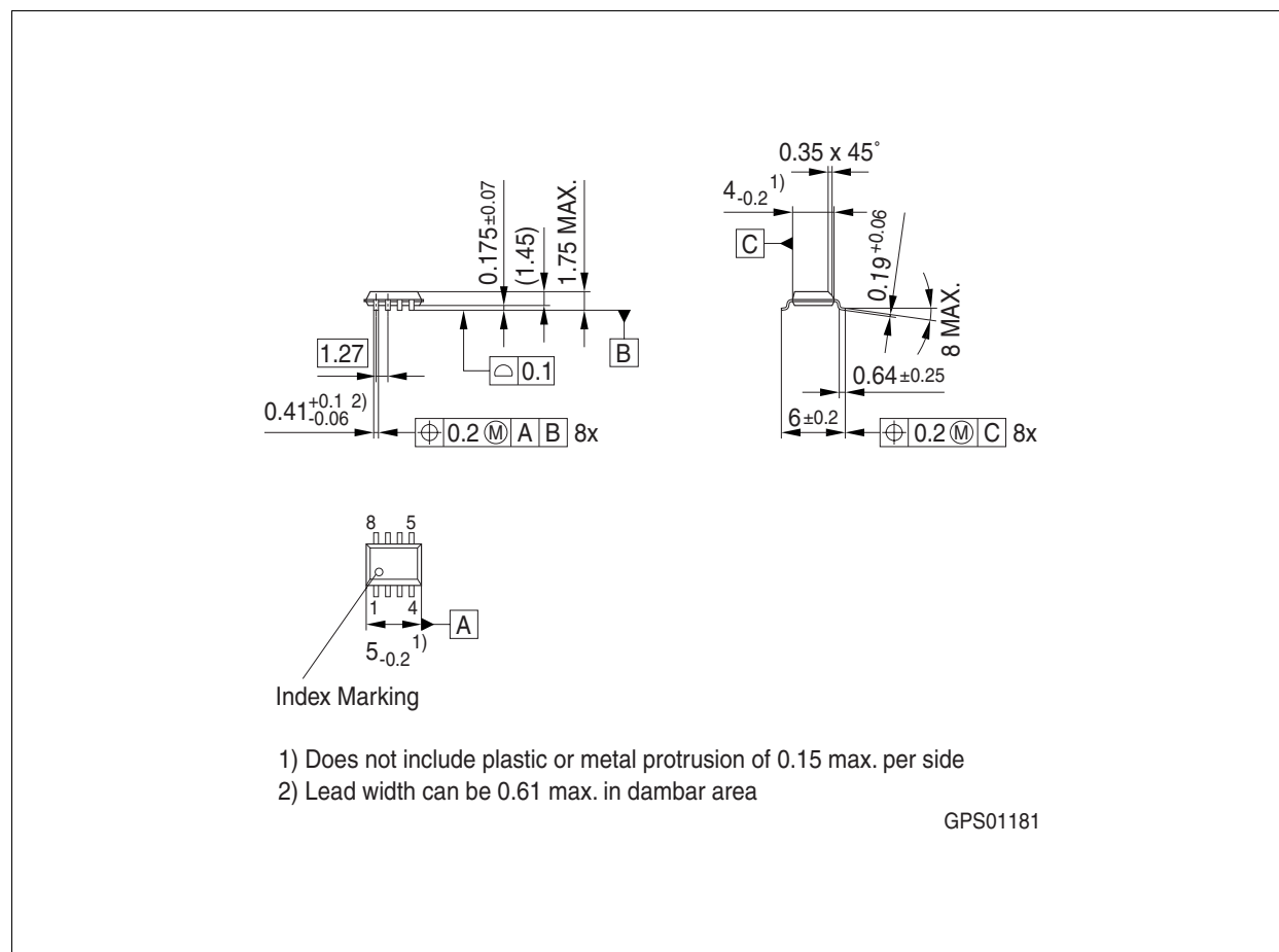
Figure 17 PG-DSO-8 (Plastic Dual Small Outline PG-DSO-8-16)
