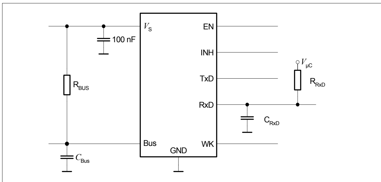
Figure 11 Simplified test circuit for dynamic characteristics
