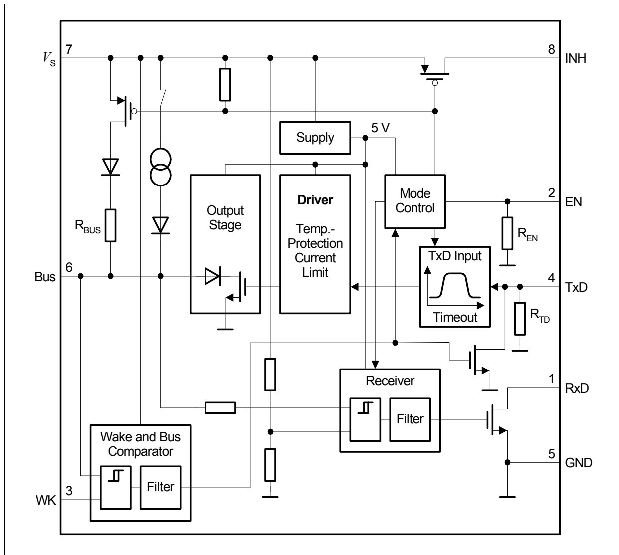
Figure 1 Block Diagram
