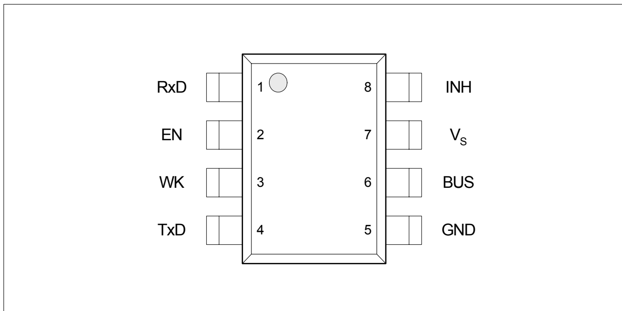
Figure 2 Pin Configuration
