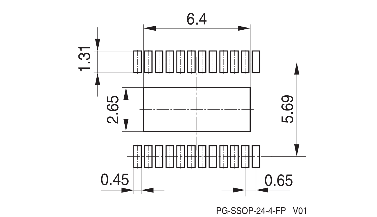
Figure 39 TLE75242-EMD Package pads and stencil
