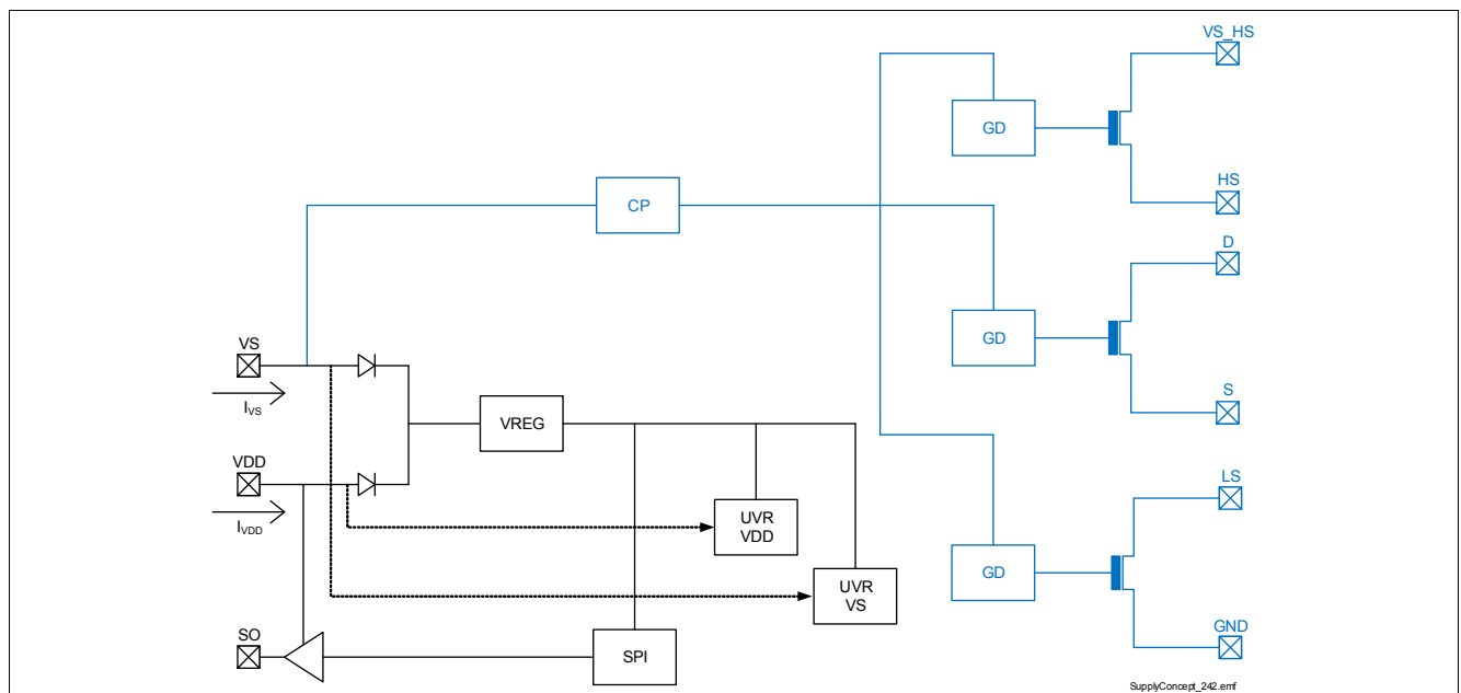
Figure 10 TLE75242-EMD Internal Power Supply concept
