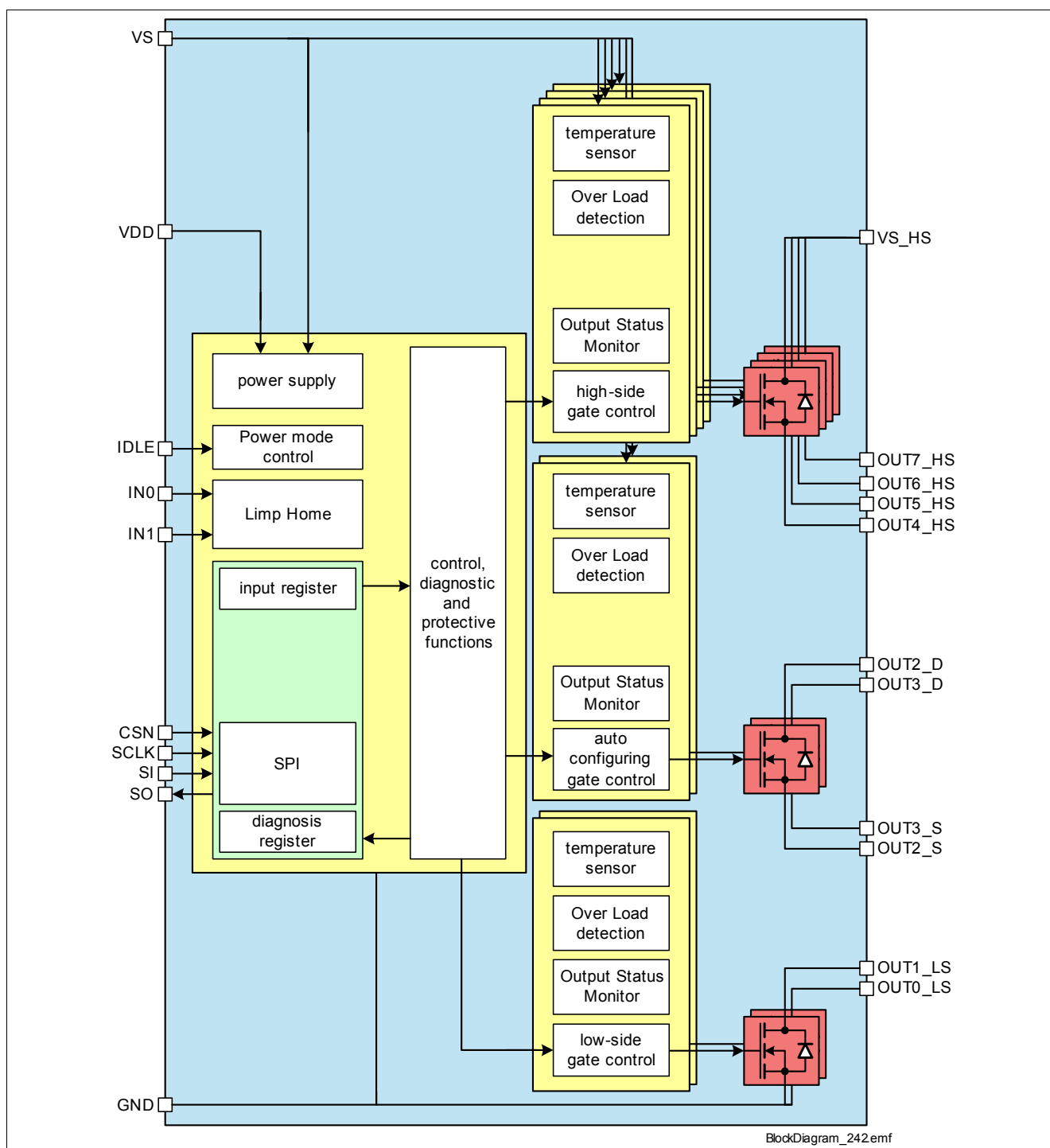
Figure 1 Block Diagram of TLE75242-EMD
