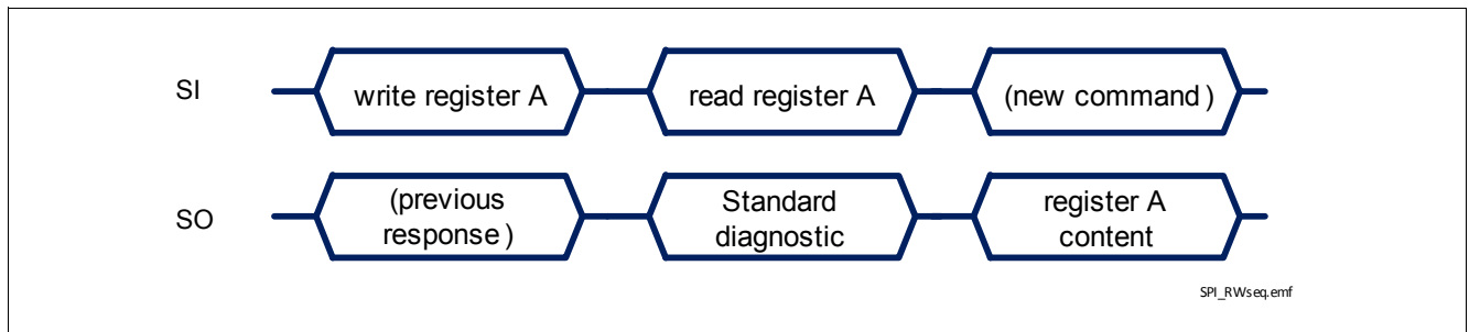
Figure 33 Register content sent back to \mu C
