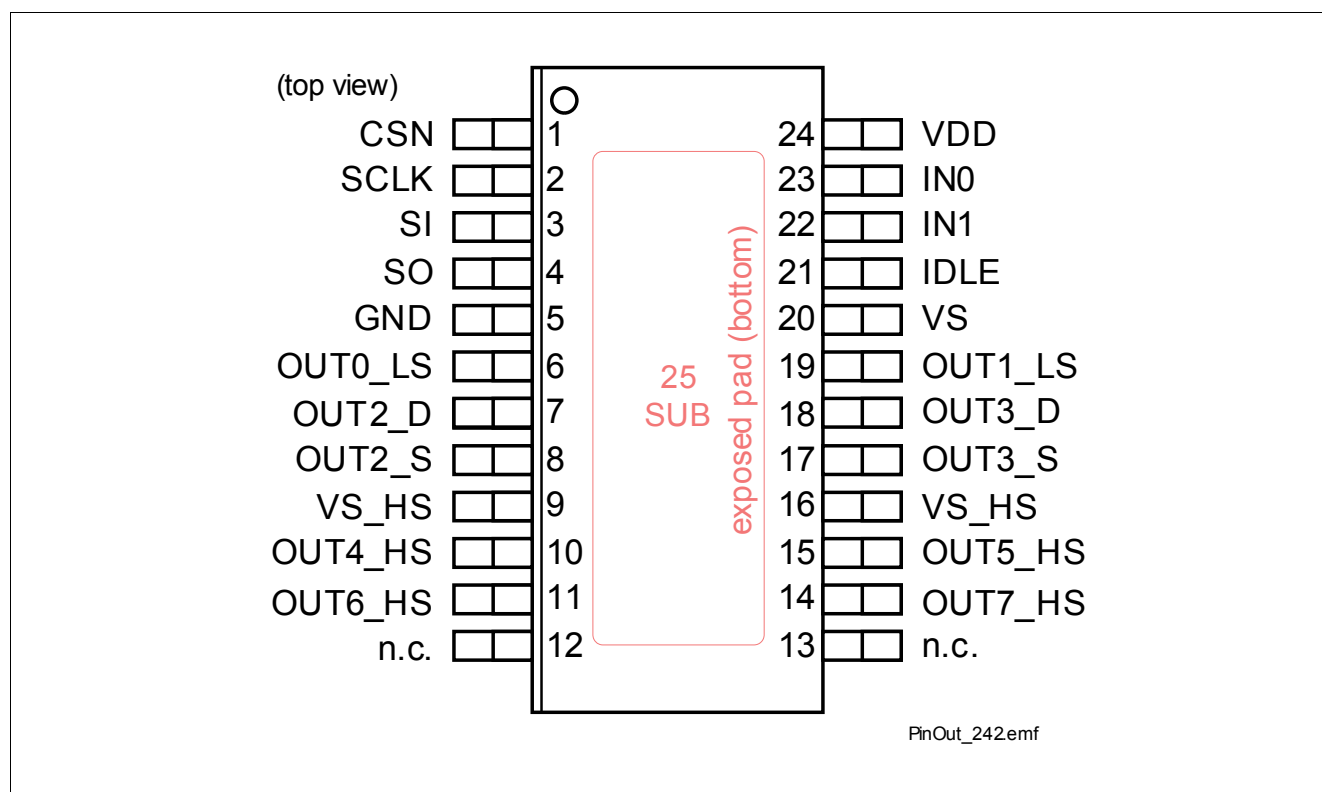
Figure 3 Pin Configuration TLE75242-EMD in PG-SSOP-24-9
