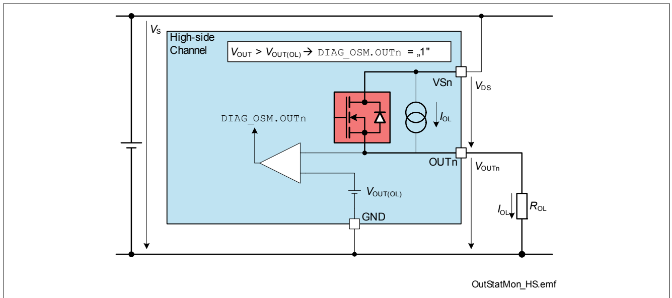
Figure 26 Output Status Monitor - concept (High-Side channels)
