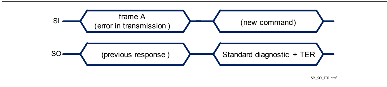
Figure 34 TLE75242-EMD response after a error in transmission
