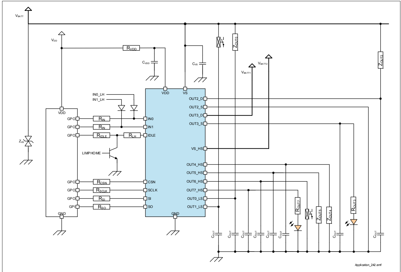
Figure 37 TLE75242-EMD Application Diagram
