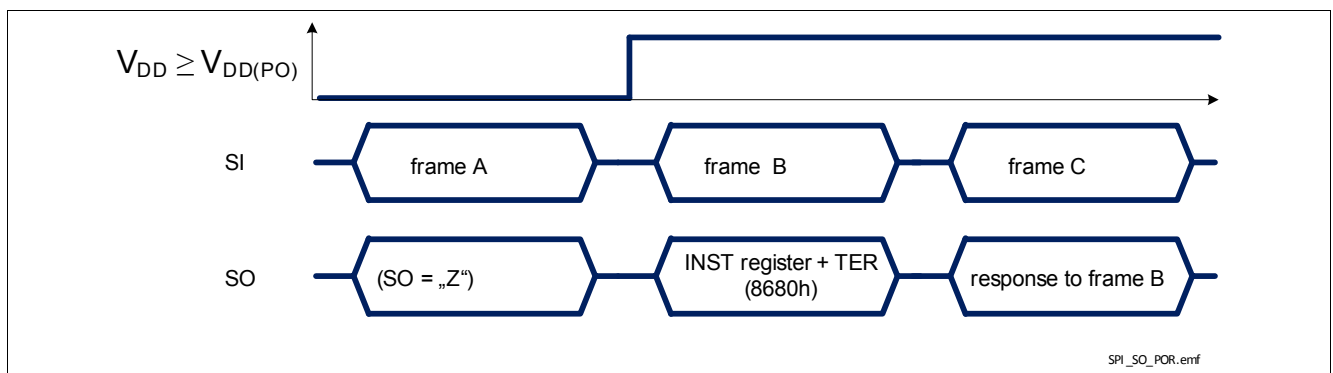
Figure 35 TLE75242-EMD response after coming out of Power-On reset at V_{DD}
