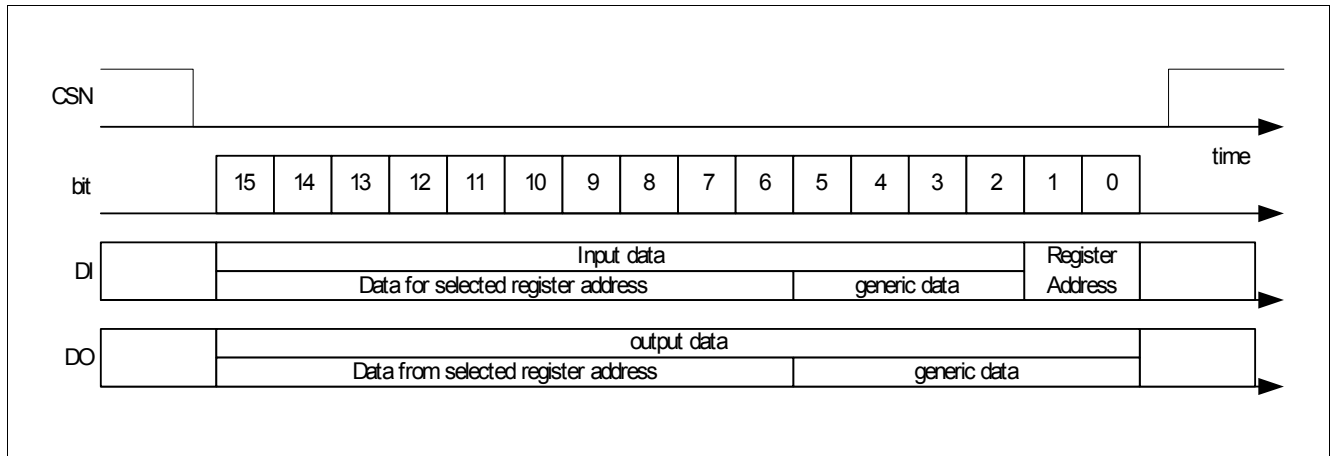
Figure 4 SPI Structure
