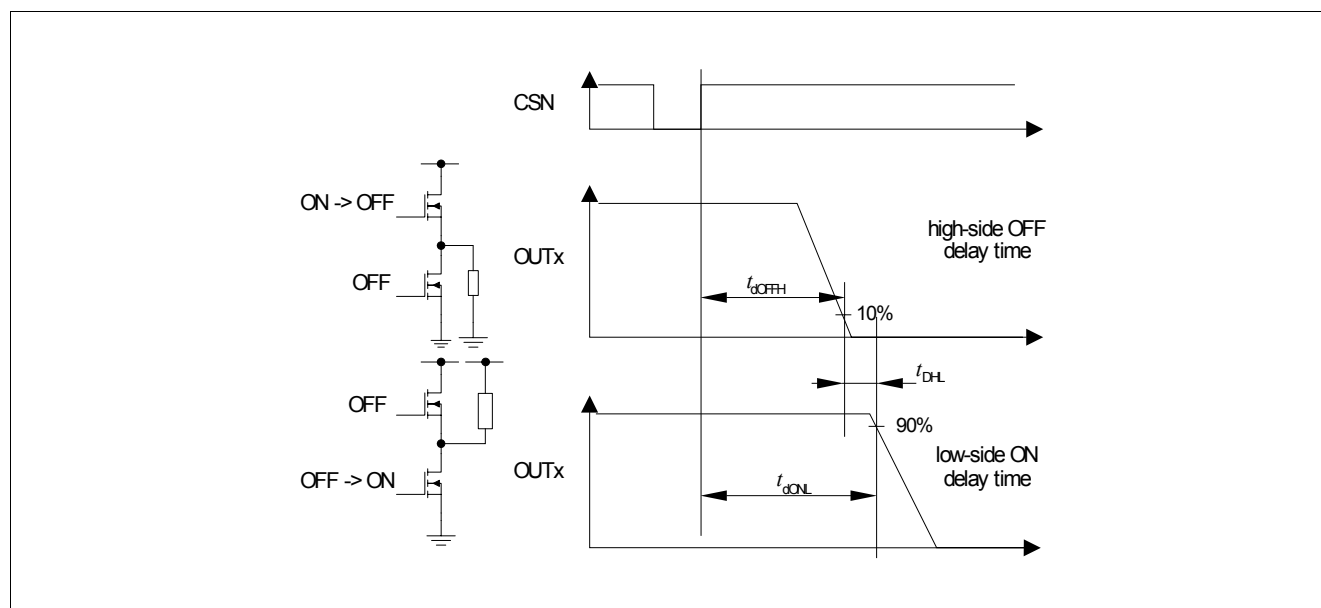
Figure 11 Timing Bridge Outputs High to Low
