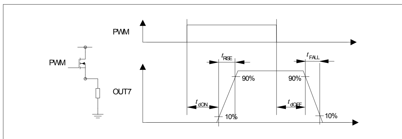
Figure 15 Timing OUT 7
