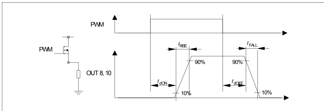
Figure 19 Timing OUT 8, 10
