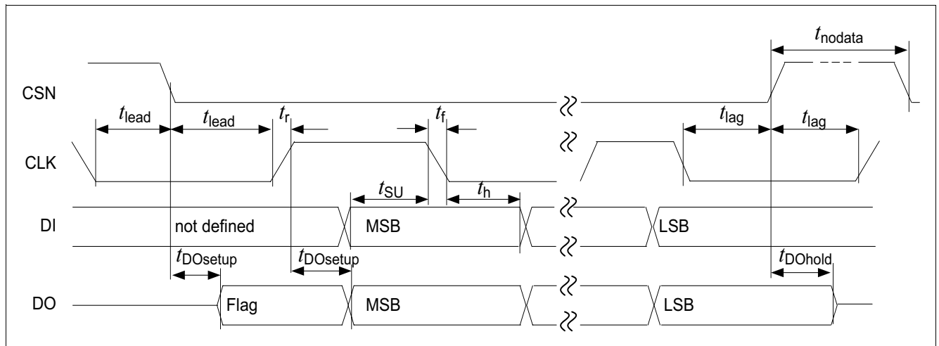
Figure 7 Timing Diagram
