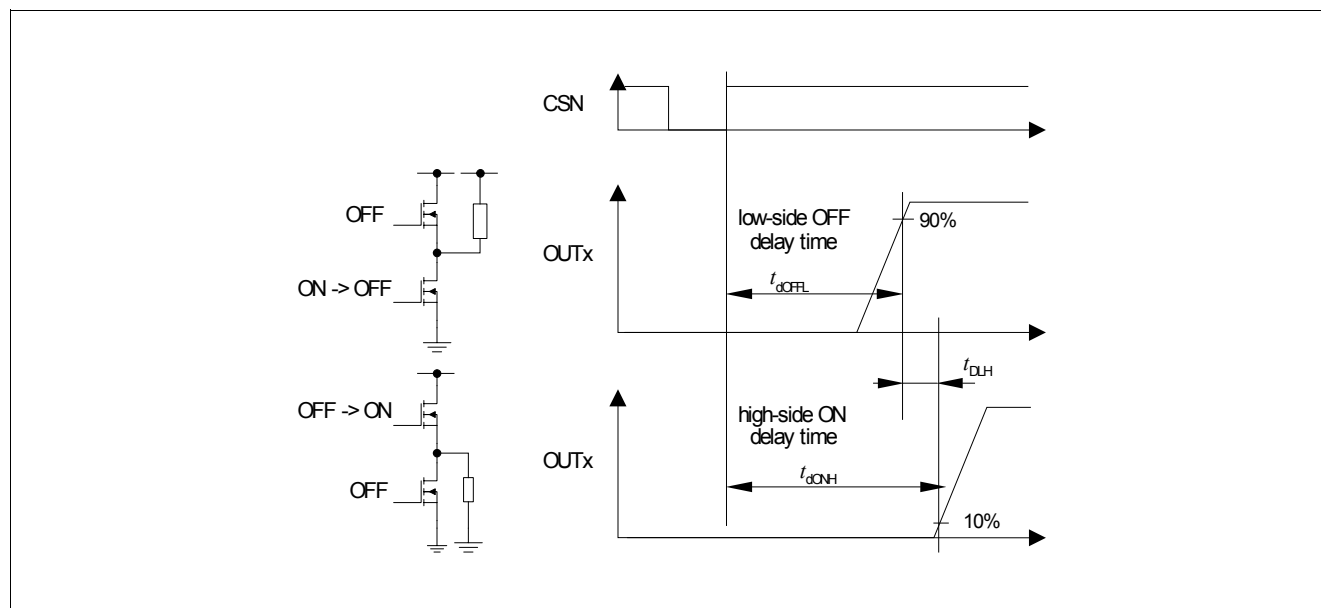
Figure 12 Timing Bridge Outputs Low to High
