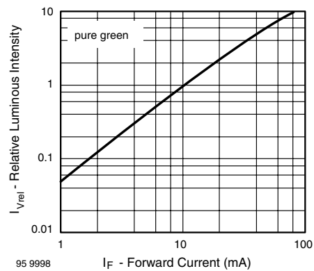
Figure 26. Relative Luminous Intensity vs. Forward Current
