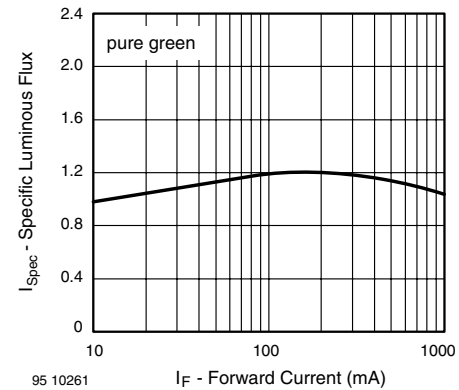
Figure 28. Specific Luminous Intensity vs. Forward Current
