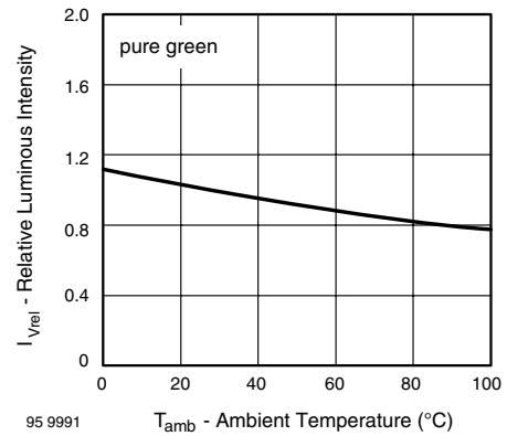
Figure 27. Rel. Luminous Intensity vs. Ambient Temperature
