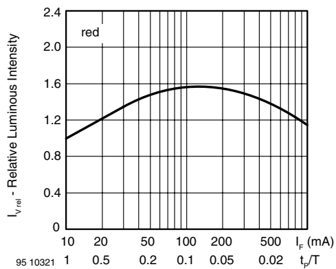
Figure 8. Rel. Lumin. Intensity vs. Forw. Current/Duty Cycle
