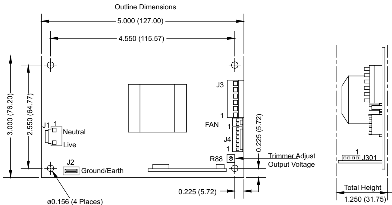
Figure 2: Mechanical Drawing
