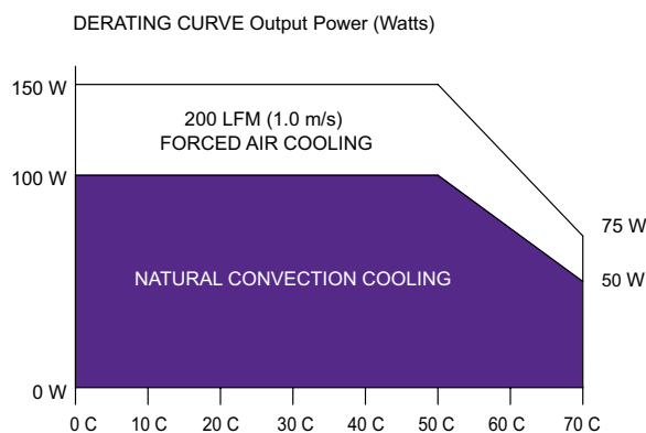
Figure 1: Derating Curve
