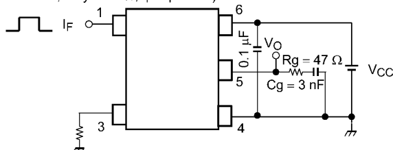
Fig. 12.1.7 Switching Time Test Circuit and Waveform
