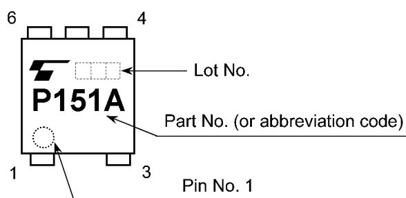
Fig. 15.1 Marking
