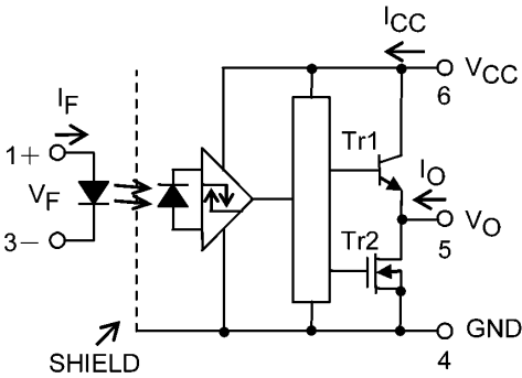
Fig. 5.1 Internal Circuit
