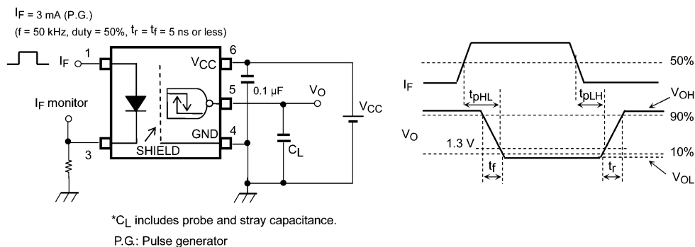
Fig. 12.1.8 Switching Time Test Circuit and waveform
