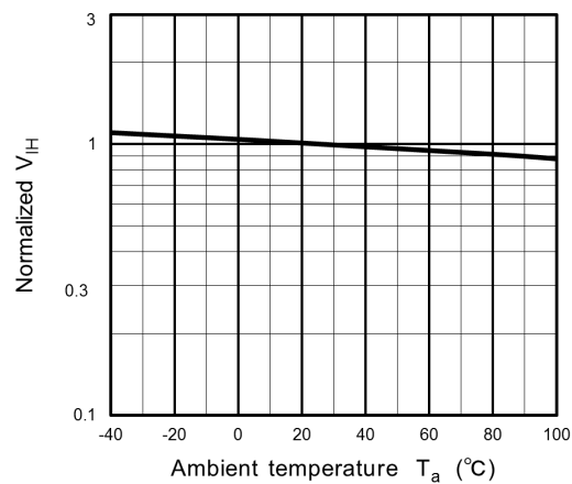
Fig. 12.10 Normalized V_{IH} - T_a
