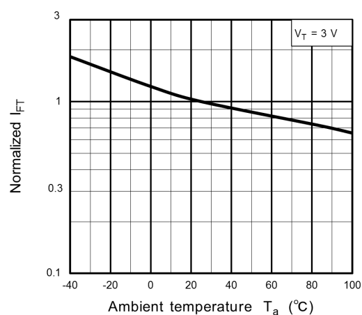
Fig. 12.6 Normalized I_{FT} - T_a
