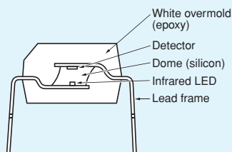
Cross section of the TLP523
