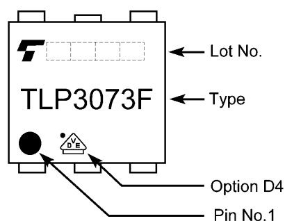
Fig. 16.4 Marking Example of TLP3073F (Note)
