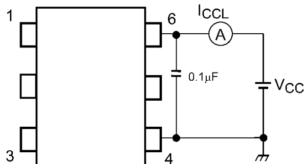
Fig. 12.1.6 I_{CCL} Test Circuit
