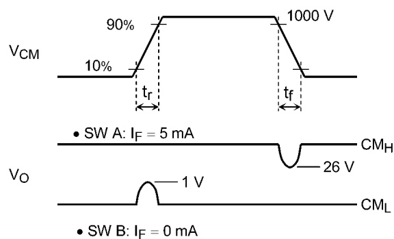
Fig. 12.1.8 Common-Mode Transient Immunity and Waveform
