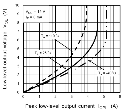
Fig. 12.2.9 V_{OL} - I_{OPL}
