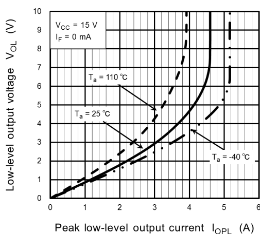
Fig. 12.2.9 V_{OL} - I_{OPL}
