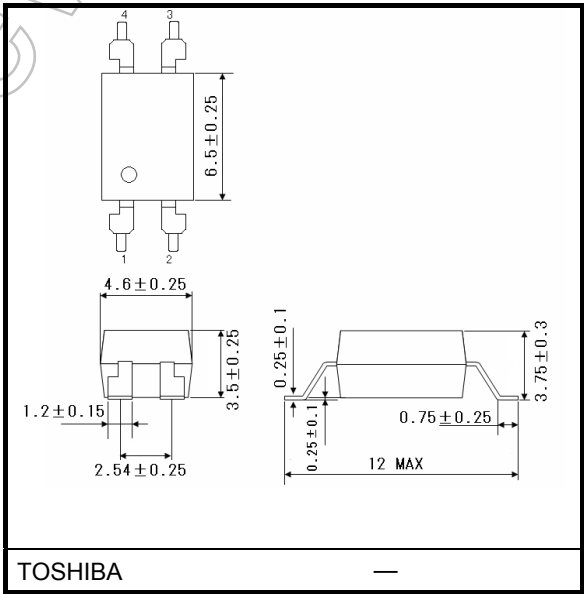
TLP781F(LF7)
