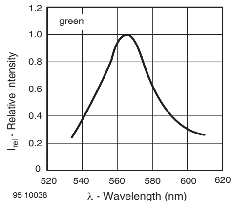
Fig. 24 - Relative Intensity vs. Wavelength
