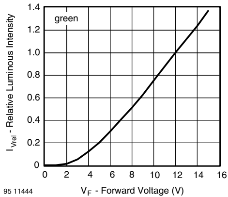
Figure 22. Relative Luminous Intensity vs. Forward Voltage
