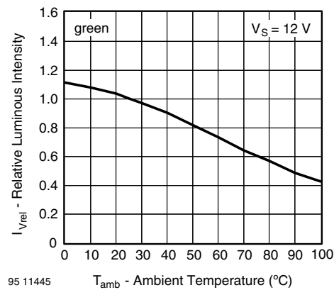
Figure 23. Rel. Luminous Intensity vs. Ambient Temperature
