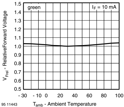
Figure 21. Relative Forward Voltage vs. Ambient Temperature
