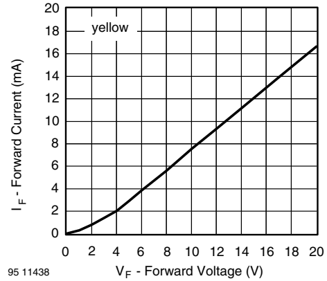
Figure 13. Forward Current vs. Forward Voltage
