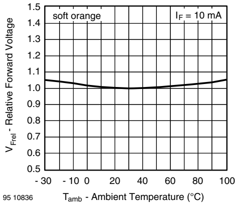
Figure 9. Relative Forward Voltage vs. Ambient Temperature
