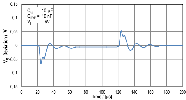
Transient Response C_{BYP} = 10 nF (TLS203B0EJV33)
