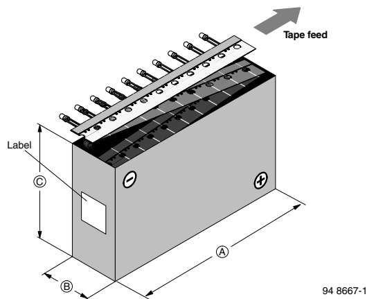
Figure 8. Tape Direction
