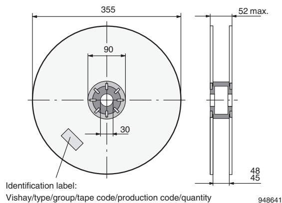
Figure 20. Reel
