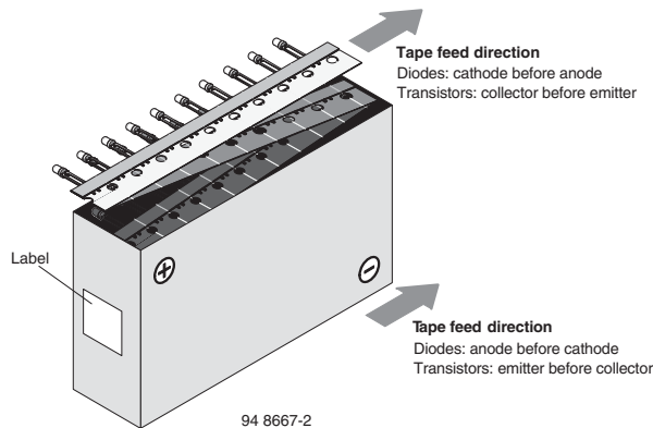
Figure 22. Tape Direction
