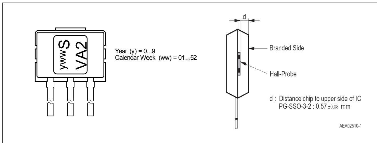
Figure 7 Marking of the TLV4946-2L and distance of the chip to the upper side
