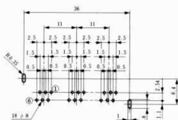
TM2RE-1818( 50 )
