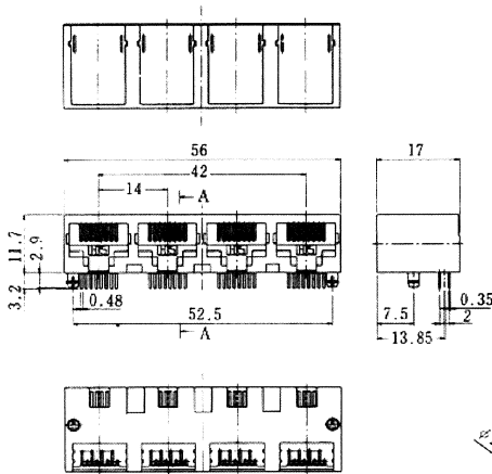
Mounting dimensions for reference (PCB mounting side)
