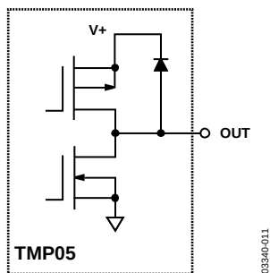
Figure 28. TMP05 Digital Output Structure
