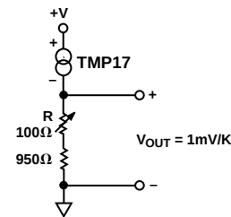
Figure 3. Basic Voltage Output (Single Temperature Trim)
