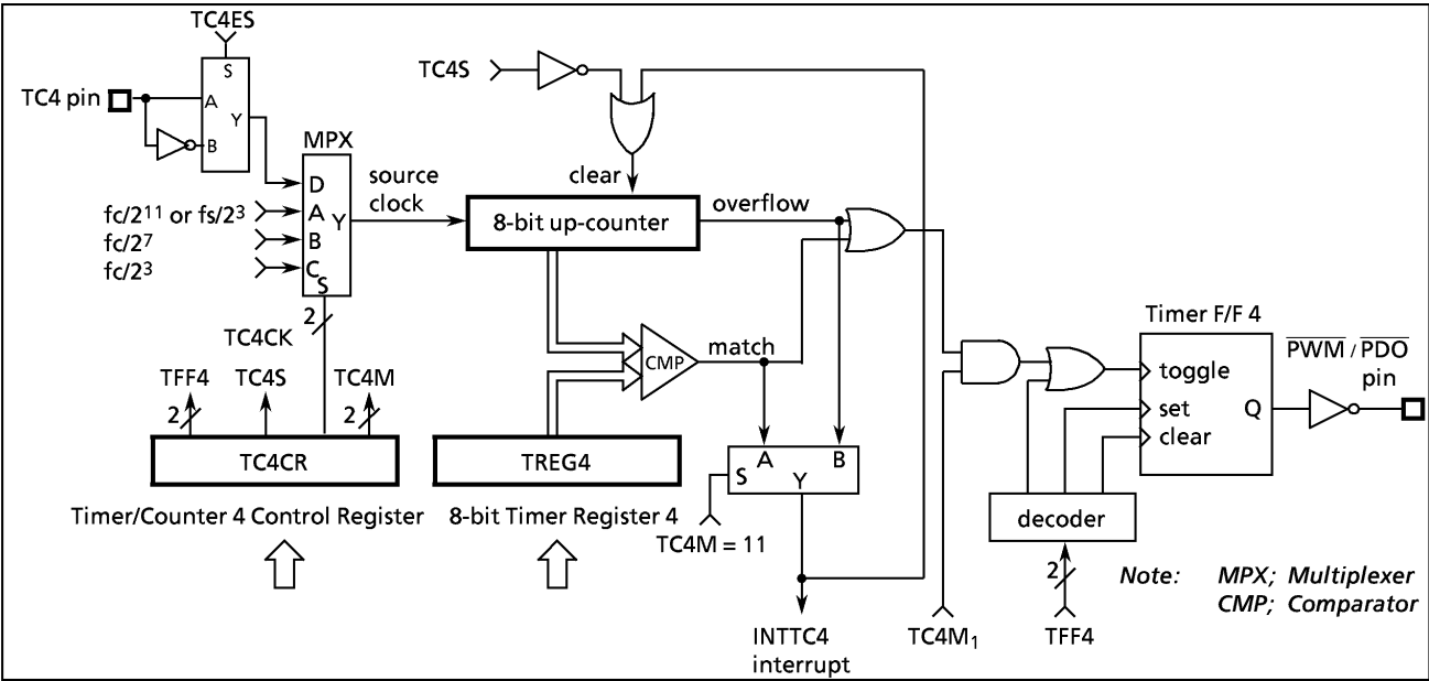
Figure 2-29. Timer/Counter 4
