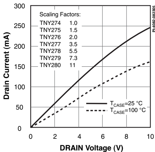
Figure 24. Output Characteristic.
