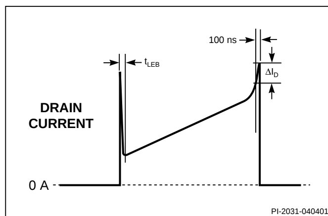
Figure 13. Example of \Delta I_D on Drain Current Waveform with Saturated Transformer.
